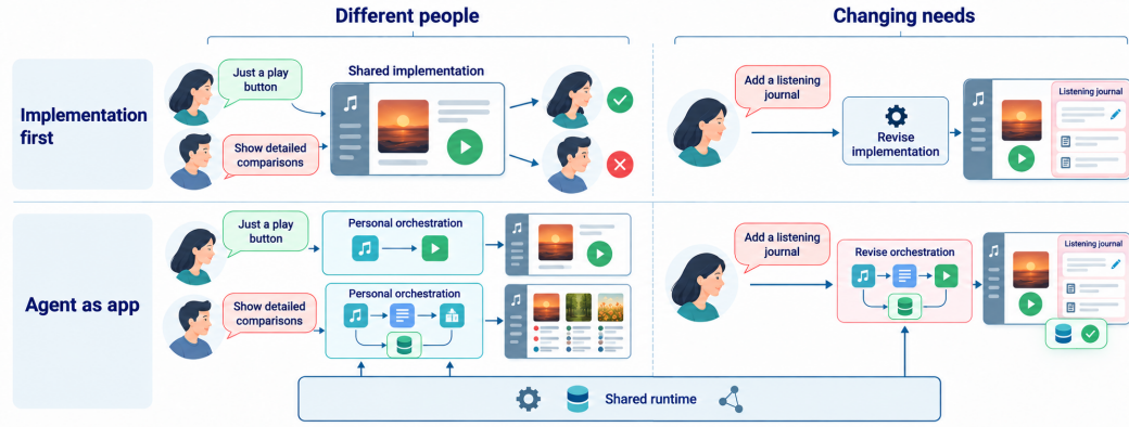
Figure 1. Agent as App connects personalization with continued use. Different listeners request a minimal player or detailed comparisons. A later request adds a listening journal that retains information alongside the original activity. The generated application must connect these goals to its interface, behavior, and saved information.
