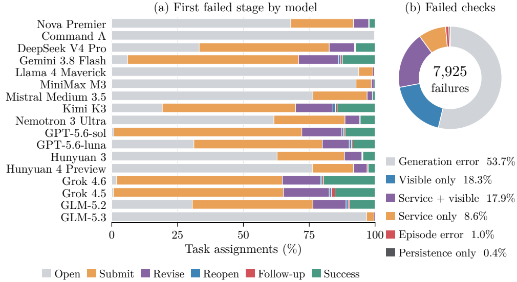
Figure 5. Failure location and recorded evidence in the original survey. (a) Each model’s 500 tasks are partitioned by the first failed native episode or success. All 17 selected models are included. Open can include a later application in a shared-world task. (b) The 7,925 failed task assignments are grouped by the failed checks in their first failed episode, with generation and episode errors separate. Service and visible categories can overlap within an episode, and the combined category keeps the displayed groups mutually exclusive. These are recorded failure patterns, not diagnoses of internal causes.
