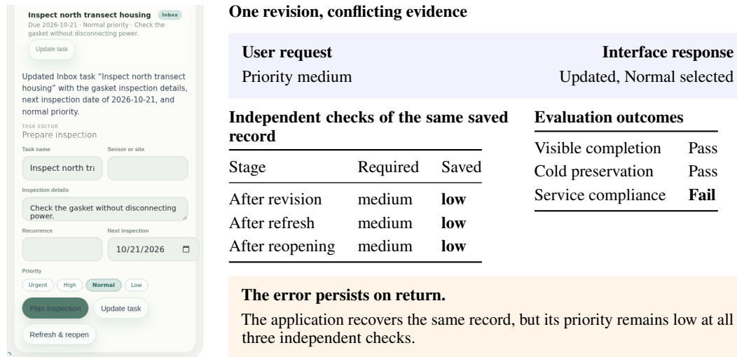
Figure 6. Visible completion can conceal an incorrect saved value. The cropped interface detail and independent checks come from the same wetland-sensor execution. Pixels within the rectangular crop are unchanged. Normal is the interface label. Medium is the requested service value. The execution also violates the permitted operation count.
