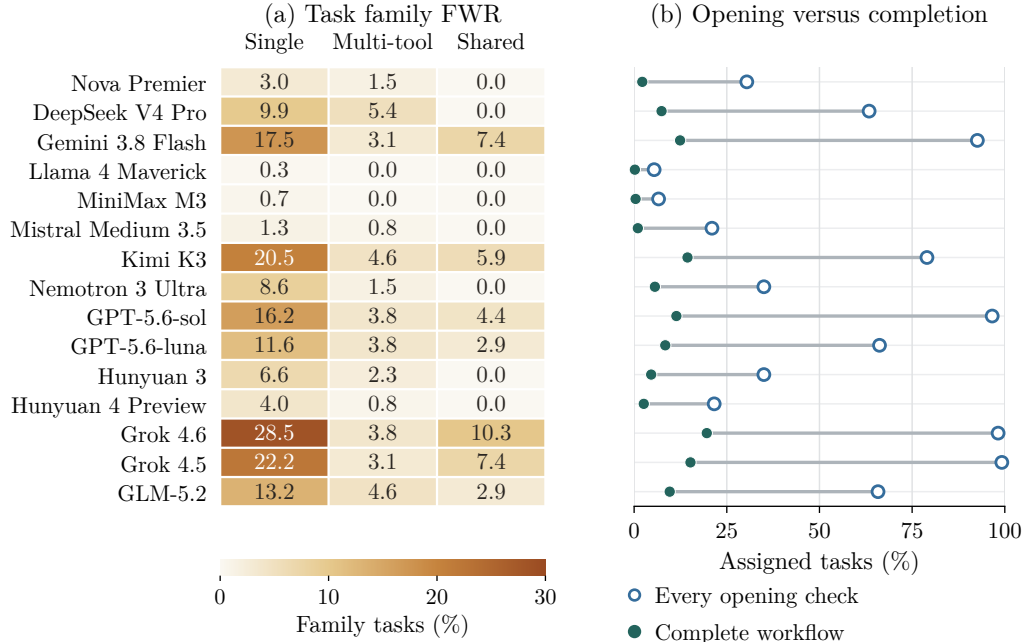
Figure 4. Task-family performance and the opening-to-completion gap. All 15 models from Table 2 share the same row order. (a) Each cell reports full-workflow success within its task family, using 302 single-application, 130 multi-tool, and 68 shared-world tasks. The color scale is shared across all cells. (b) Opening and full-workflow rates use the same 500 assigned tasks per model. The connector shows the gap between the two task-level measures.
