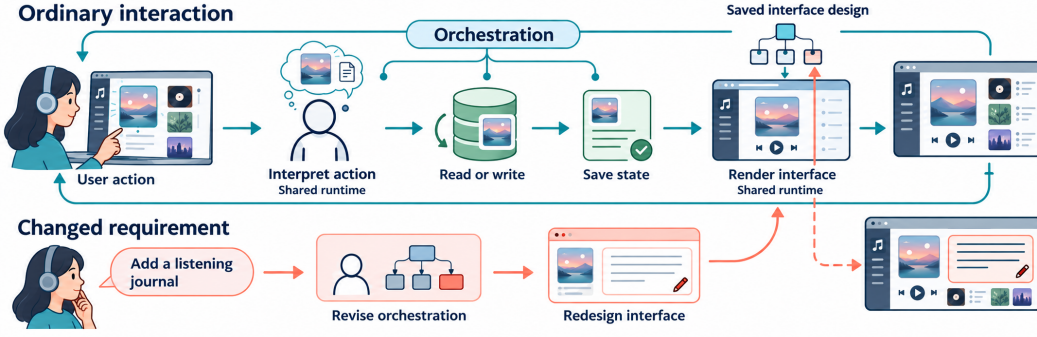
Figure 3. A task-specific orchestration links interface elements, action goals, and saved information. The shared runtime interprets submitted inputs, uses services, saves the result, and renders the resulting interface. The application keeps its identity as the user continues the workflow.
