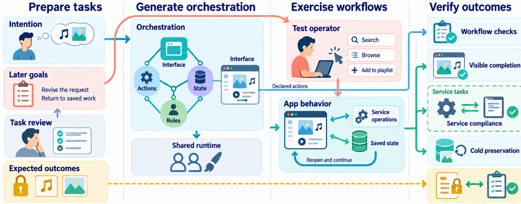
Figure 2. The evaluation workflow. Prepare an intention, later goals, and expected outcomes. Generate an orchestration from the intention and permitted context. Execute ordered goals through declared actions or the rendered interface. Check workflow completion, visible outcomes, and preserved state. Service tasks additionally verify saved records independently. The test operator supplies user actions. The application-side agent interprets them and carries out the requested operations.
