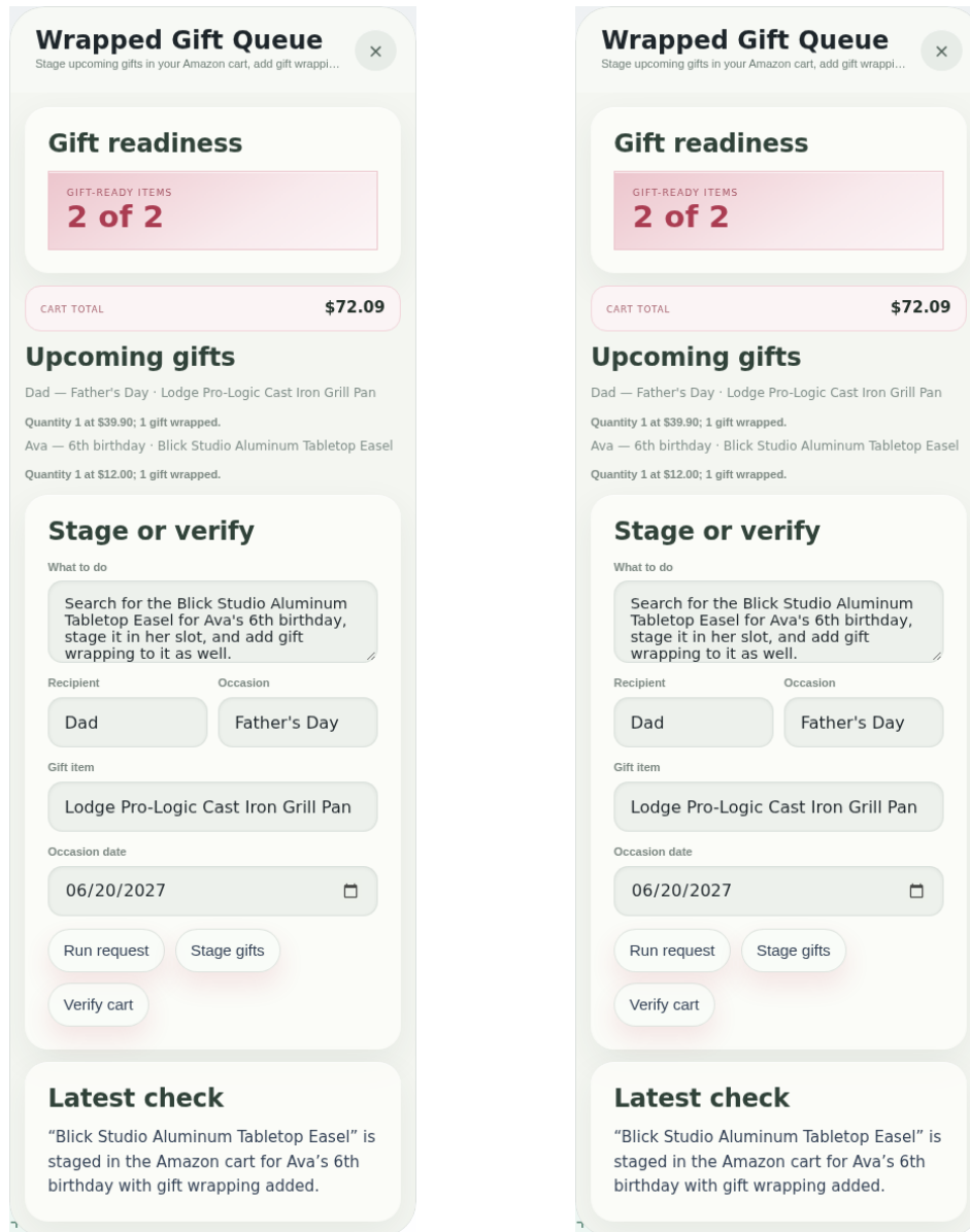
Figure 9. Amazon gift queue. Continued. The queue now shows wrapped gifts for Dad and Ava. The separate recorded reopening capture is pixel-identical to the post-request capture. Complete original screenshots are reproduced without retouching.
